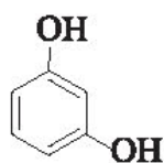
benzene-1,2-diol (resorcinol)
