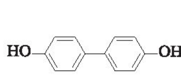
biphenyl-4,4'-diol
