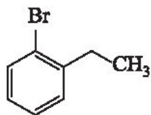
1-bromo ethylbenzene
