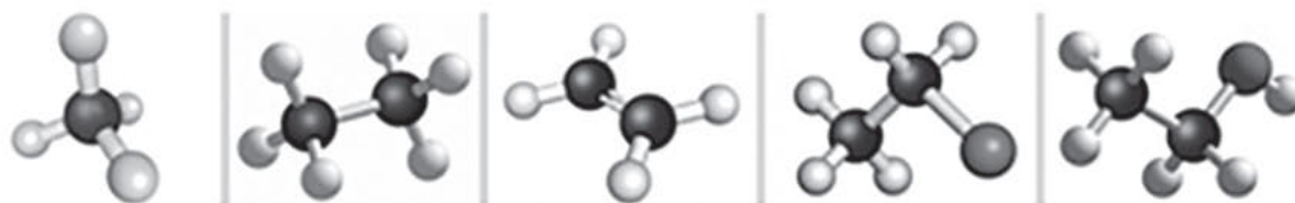
methane
