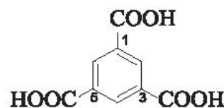
benzene-1,3,5-tricarboxylic acid
