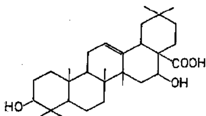
Acid echinocystic
