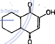
Lawson (hydroxyl 2-naphthoquinone 1-4)
