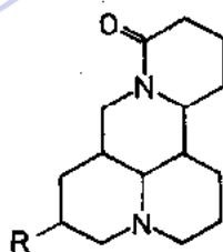
Matrin C_{15}H_{24}N_2O
