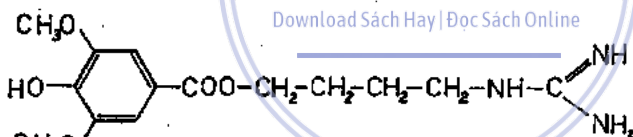
Leonurin
