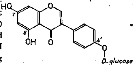
Sophoricosid
