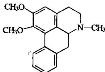
Nuciferin
