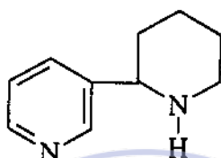
Anabasin
