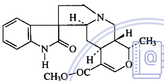
Mitraphyllin
