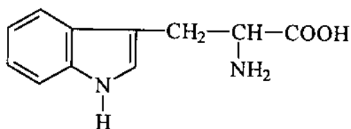
Tryptophan
