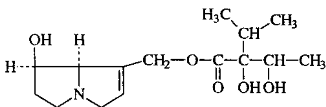
Indicin
