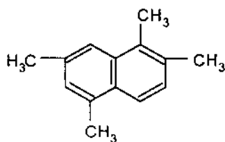
Sapotalin
