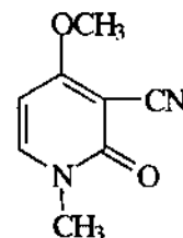
Ricinin
