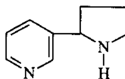
Nor-nicotin
