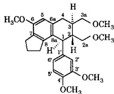
Hypophylanthin
