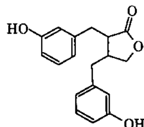
Enterolacton
