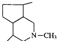
Skythanthin
