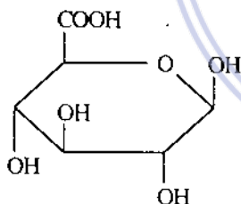
Acid glycuronic
