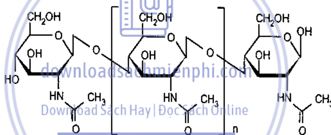
Chitin
