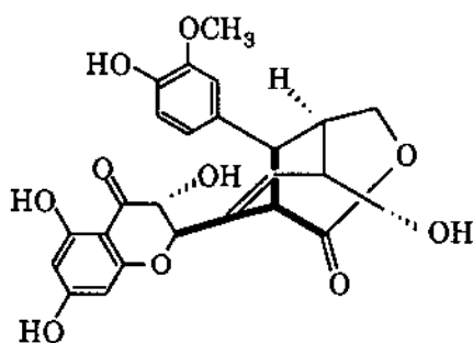
Silydianin
