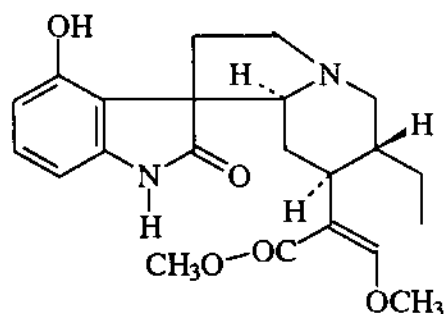
Rotundifolin
