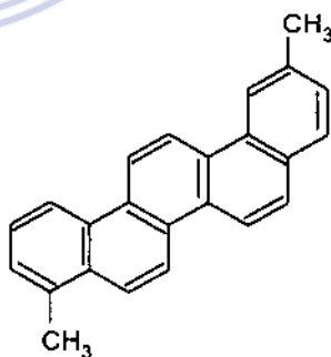
Dimethylpixin
