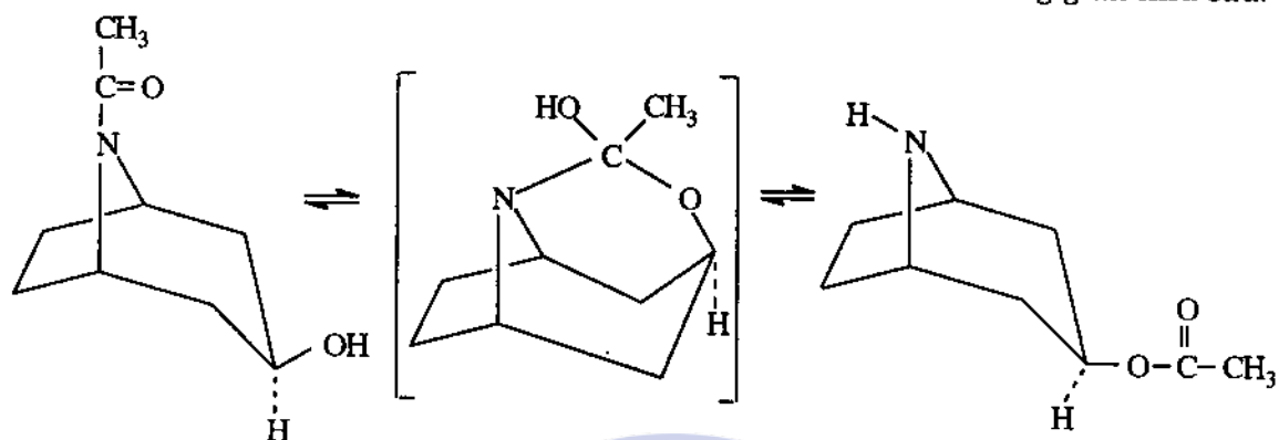
N-acetyl-norpseudotropin
