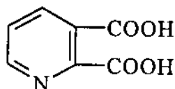
A. quinolic
