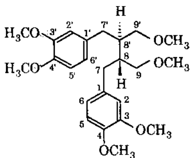
Phylanthin
