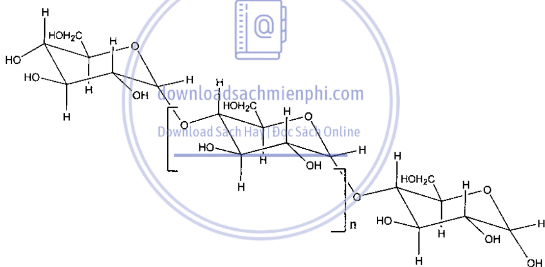
Amylose
