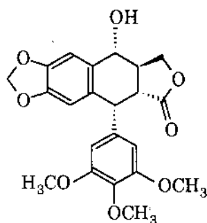
Podophylotoxin
