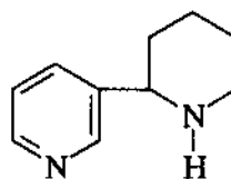
Anabasin
