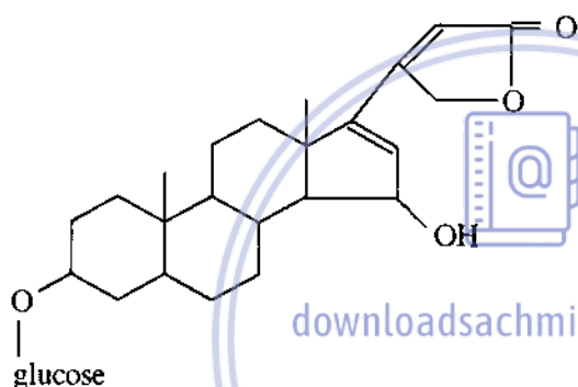
Neriantin
