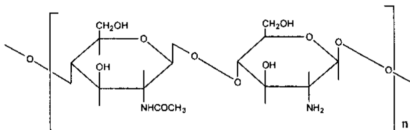
Chitosan
