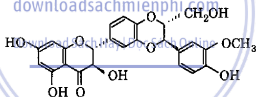
Silybin
