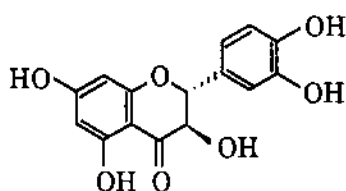
Taxifolin
