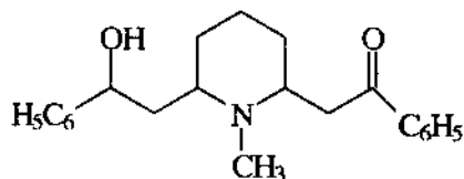
Lobelin
