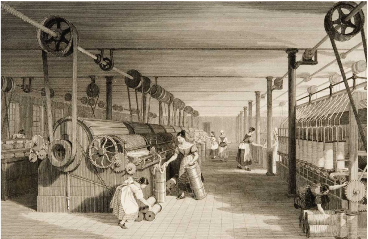
MECHANICAL LOOMS
