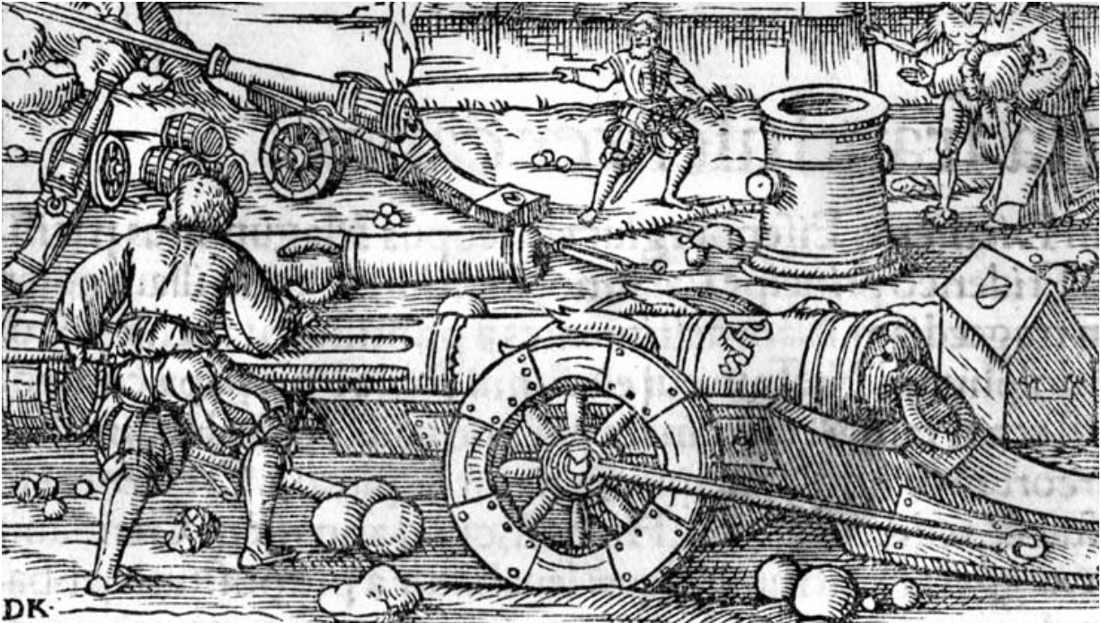
SIXTEENTH-CENTURY CANNON
