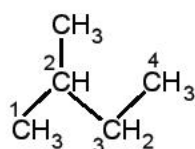
2-methylbutane
