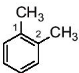
1,2-dimethylbenzene ( o -xylene)
