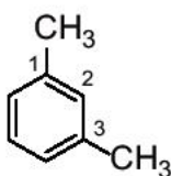
1,3-dimethylbenzene ( m -xylene)
