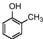
o-cresol
