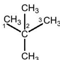
2,2-dimethylpropane (neopentane)
