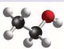
ethanol
