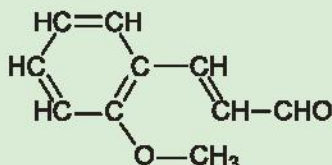
o-methoxycinnamaldehyde
