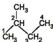
2-methylbutane (isopentane)
