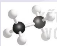
ethane
