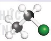
ethyl chloride
