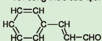
cinnamaldehyde
