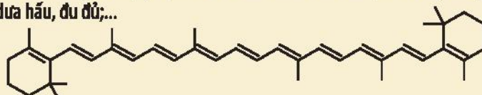
β-carotene
