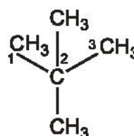
2,2-dimethylpropane (neopentane)
