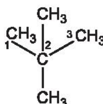
2,2-dimethylpropane (neopentane)
