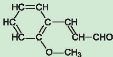
o-methoxycinnamaldehyde
