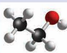
ethanol
