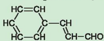
cinnamaldehyde
