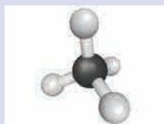
methane
