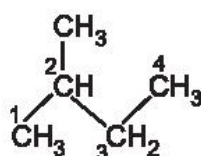
2-methylbutane (isopentane)
